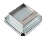
1 Compartment (125x125x56mm)
