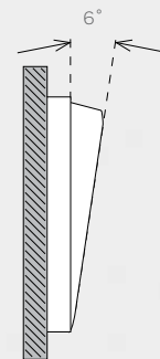
Conventional rocker
